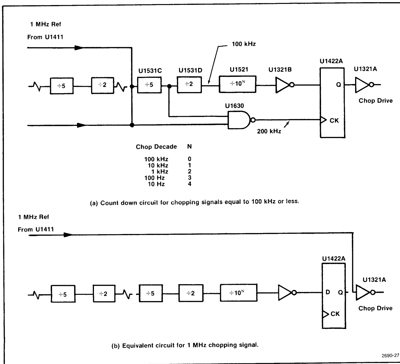
Fig. 4-14. Divider chain configurations for chopping signals.
